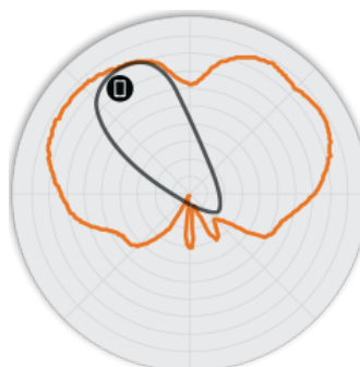
Figure 4. 7781-CM 2.4GHz Elevation Antenna Patterns
