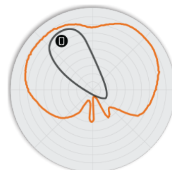
Figure 5. 7781-CM 5GHz Elevation Antenna Patterns
